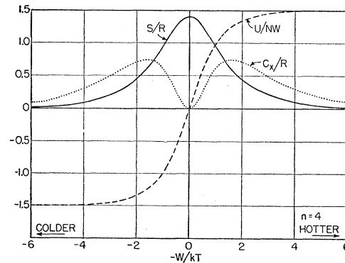
FIG. 2. The internal energy, the entropy and the specific heat are plotted as a function of -1/T measured in units of k/W for the same system as Fig. 1. As discussed in Sec. II this choice of abscissa corresponds to the colder points being to the left of the hotter ones. The dashed curve (---) is for the internal energy U , the full curve (—) is for the entropy S , and the dotted curve (····) is for the specific heat C_x .
